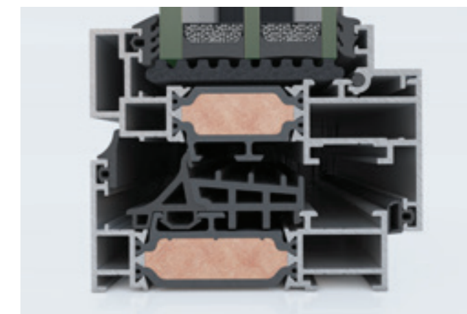
ELVIAL I 2 _ INNOVATIVE INSULATION TECHNOLOGY FOAMED EPDM GASKET INSULATION FOAM INSULATING PROFILE
