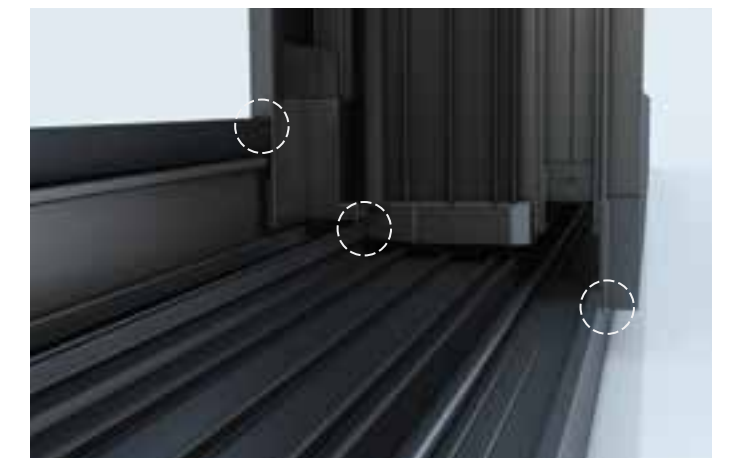
EPDM ADJOINING PROFILE END CUP The EPDM adjoining profile end cup ensures excellent waterproof performance, even on double sash typologies.
