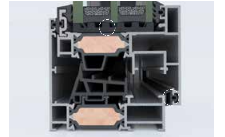
CO-EXTRUDED GASKET & FOAM INSULATING PROFILE Co-extruded gasket is used in the perimetrical area of the window, improving energy performance. Whilst foam insulating profile is fitted below the glazing zone, minimizing thermal energy loss.
